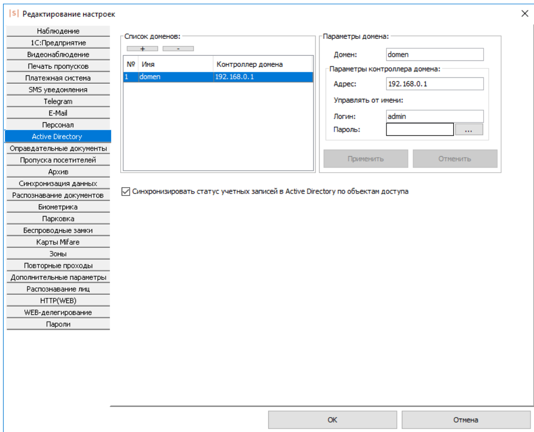
Настройки Active Directory.
